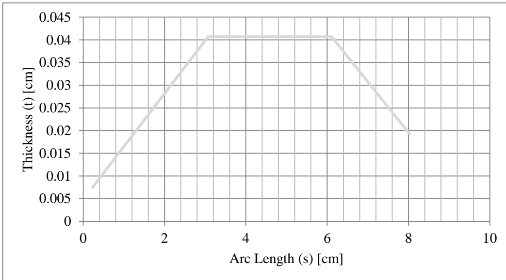
Fig. 6.12. Linearized LEU fuel thickness profile. Overall, the LEU fuel profile is thinner than the HEU profile. Even though the LEU fuel has less U^{235} per weight than the HEU fuel, it has a higher density.
