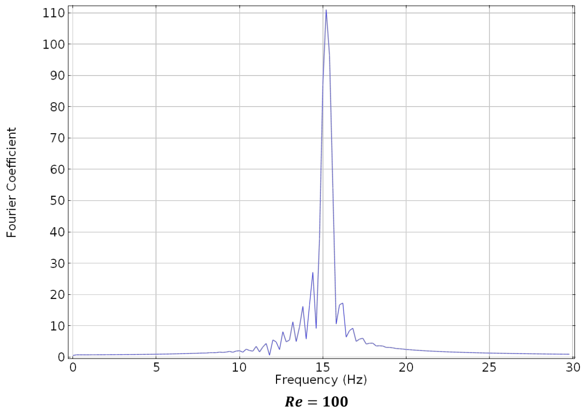
Fig. 4.8. FFT of the C_l for the stationary cylinder (part 1 of 2).
