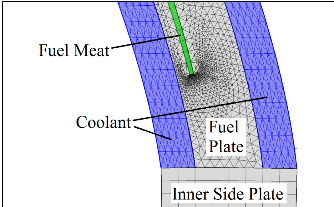
Fig.5.13. Fueled section cross-sectional mesh. Structured quadrilateral mesh elements in the coolant region have been converted to triangular elements in order to facilitate meshing between axial coolant components.
