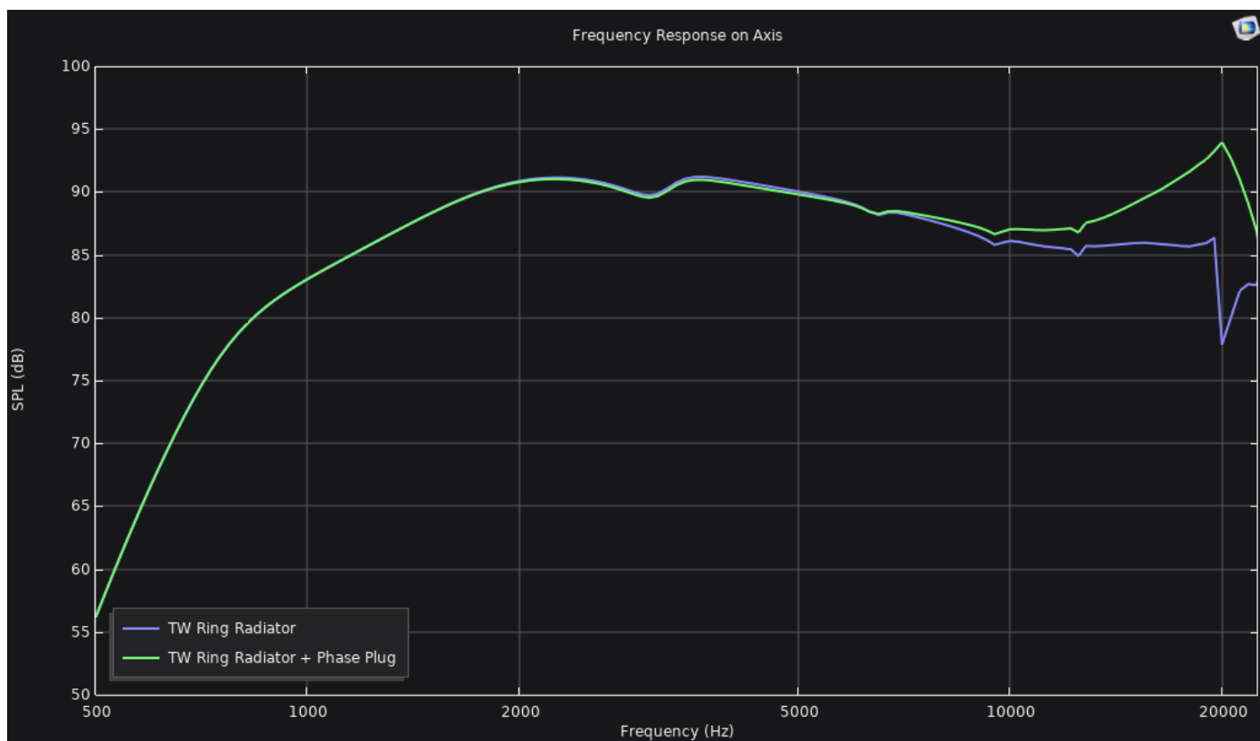
Figure 3 : Frequency Response on Axis
