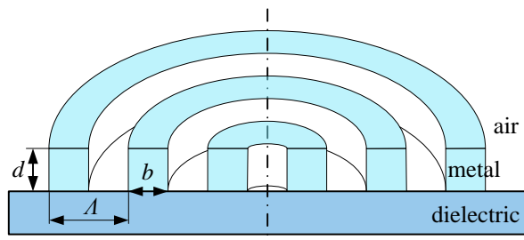
Sectional view of circular grating
